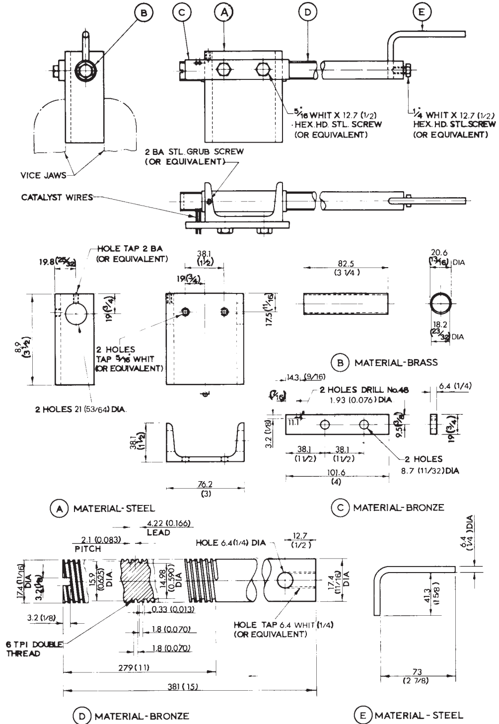
Dimensions are in millimetres (inches). FIG. 3 Mandrel for Winding Catalyst Coils
