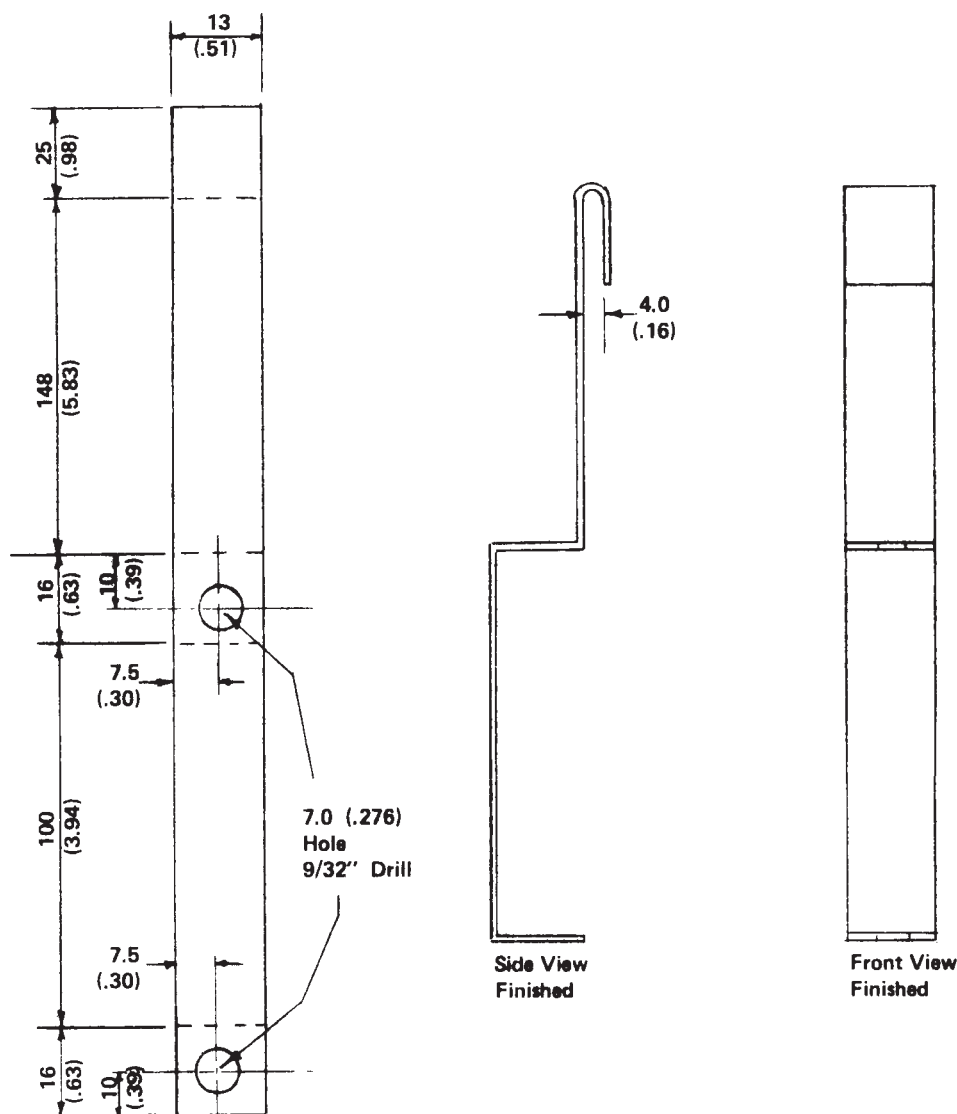
FIG. 2 Thermometer Bracket
