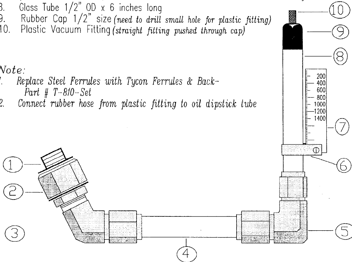
FIG. A2.24 Oil Level Measurement Setup
