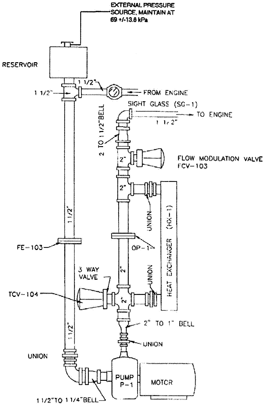
FIG. A2.2 Typical Engine System in Air-To-Close Configuration
