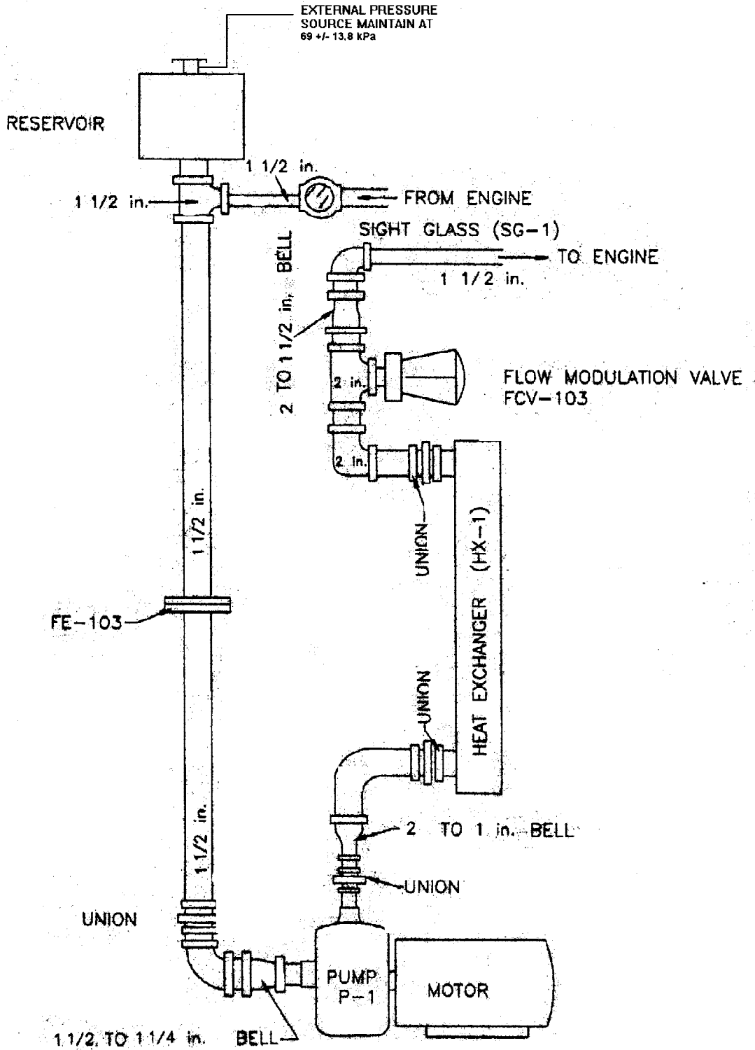
FIG. A2.3 Alternative Engine System Configuration
