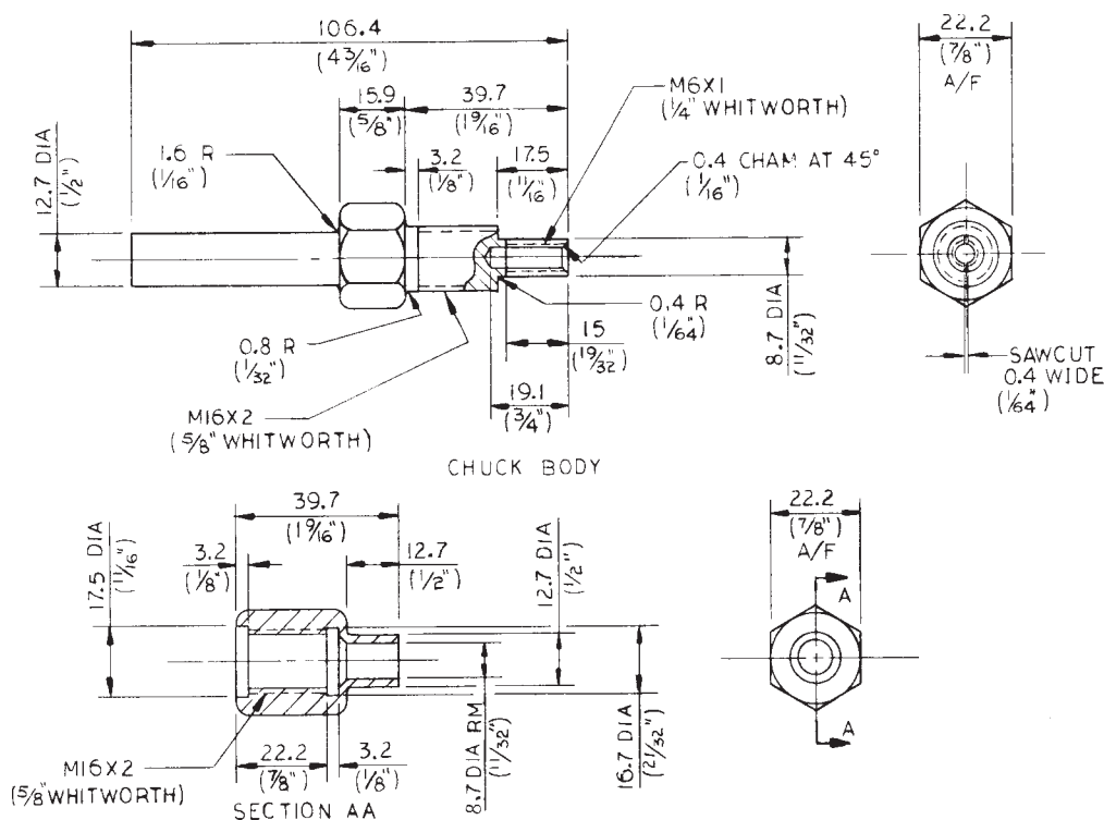
FIG. 4 Chuck for Polishing Test Rods
