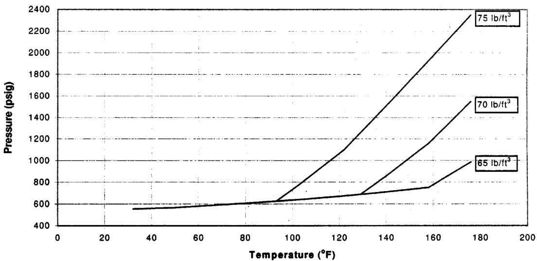
FIG. 3 Isometric Diagram of HFC-236fa Pressurized to 600 psig (42.4 bar) with Nitrogen at 72°F (22°C)
