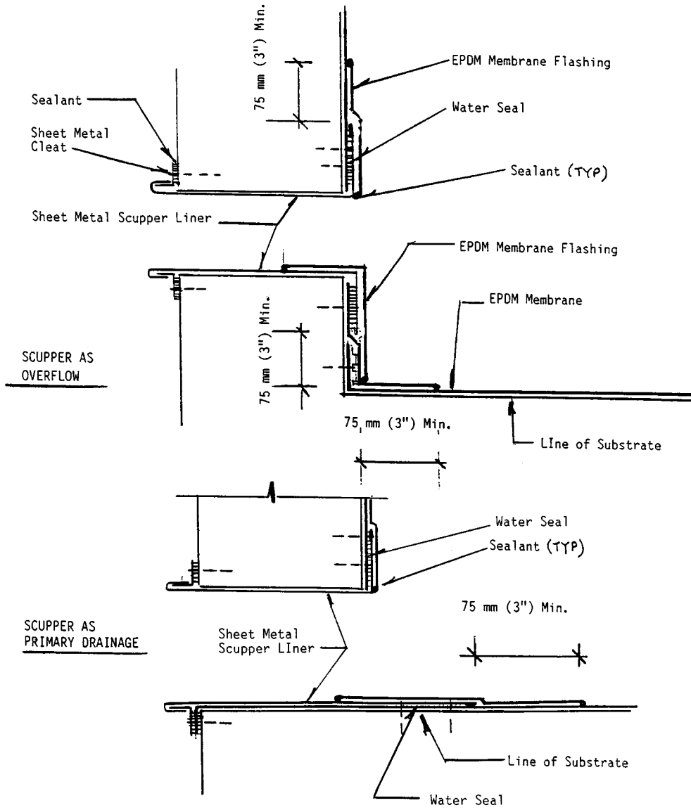
FIG. 7 Scuppers
