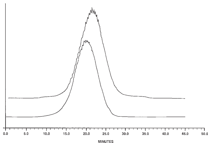
FIG. X1.6 High Temperature Simulate Distillation Chromatogram of a Heavy Distillate Fraction (HTSD-95-6) Obtained on a (50 % Phenyl) Methylpolysiloxane and 100 % Dimethylpolysiloxane
