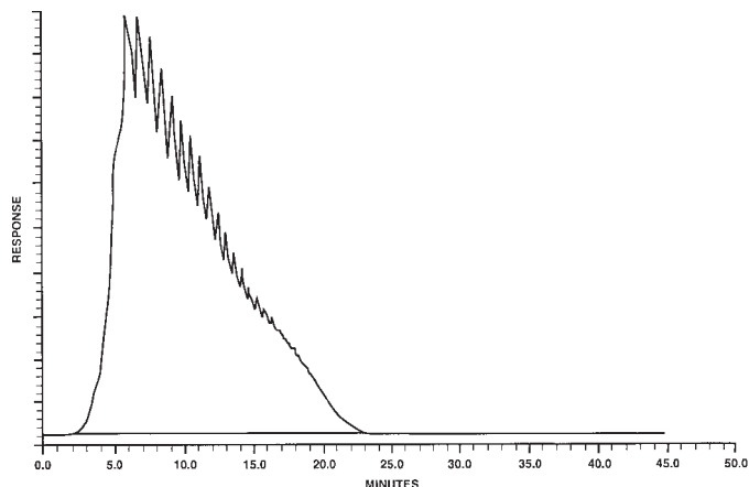
FIG. 4 Chromatogram of Round Robin Sample 95-3 Obtained Using a Fused Silica Capillary Column with 100 % Dimethylpolysiloxane Stationary Phase
