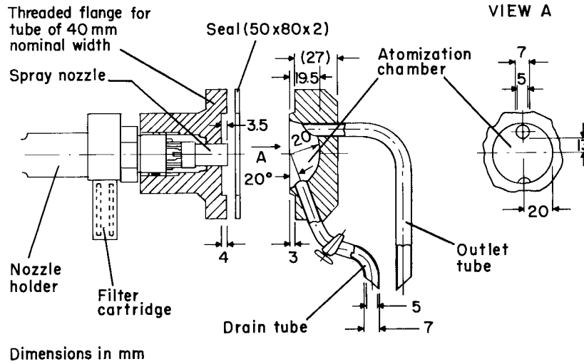
FIG. A1.3 Atomization Chamber with Spray Nozzle and Nozzle Holder
