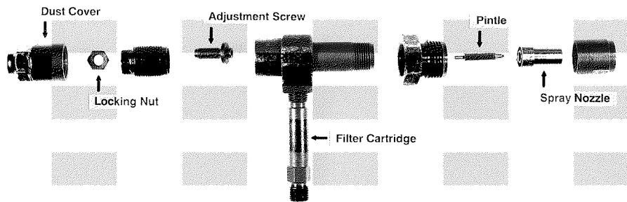
FIG. A1.4 Spray Nozzle and Nozzle Holder
