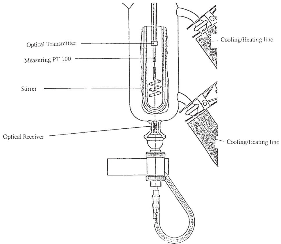
FIG. A1.3 Optical Scheme
