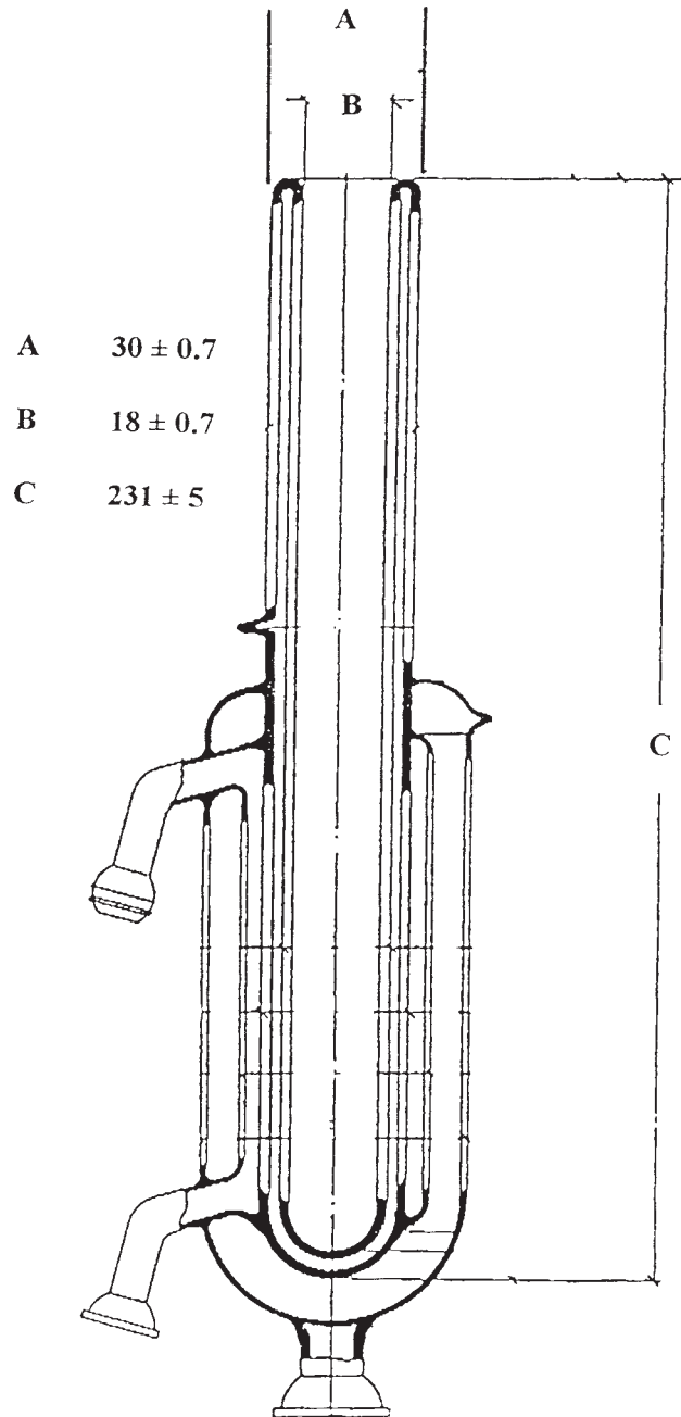
FIG. A1.1 Test Chamber
