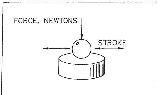
FIG. 2 Test Specimen Diagram
