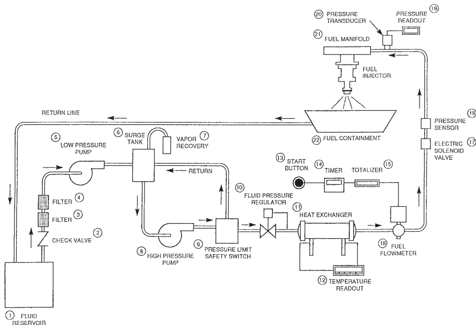
FIG. 1 Fuel Injector Flow Apparatus (example)
