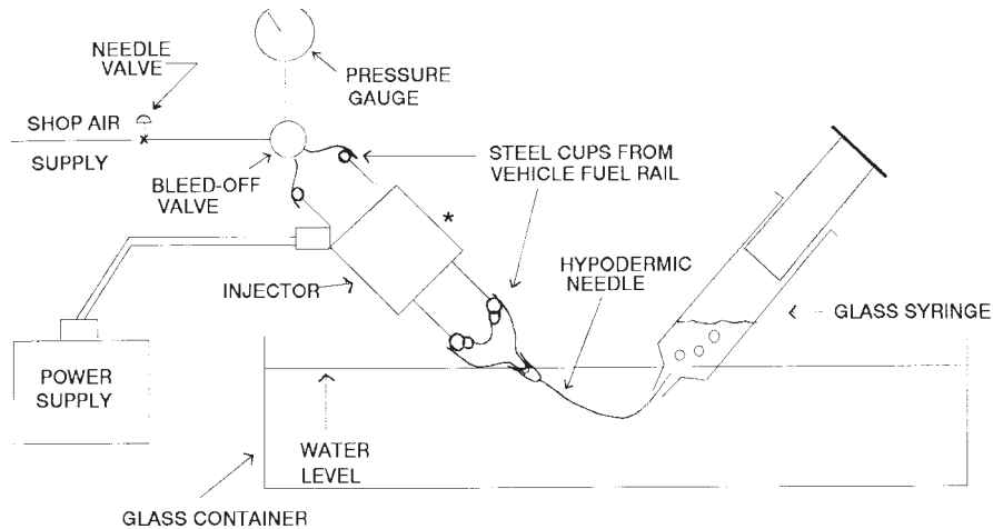
FIG. A1.1 Injector Leak Test Apparatus A
