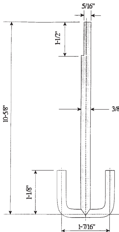
FIG. 1 Stainless Steel Agitator
