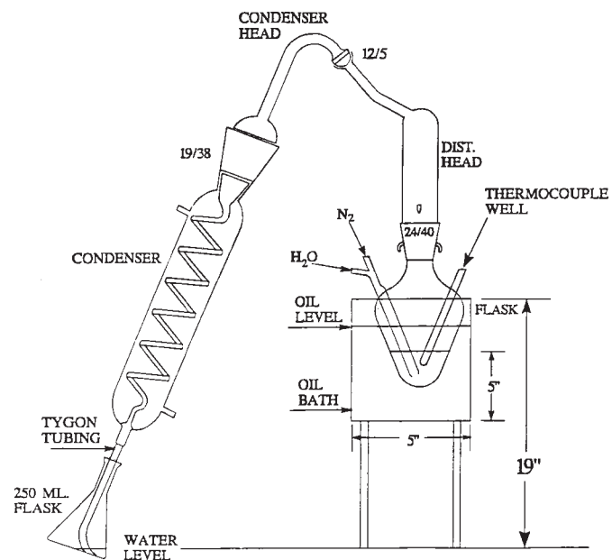
FIG. 2 Oxidation and Distillation Apparatus
