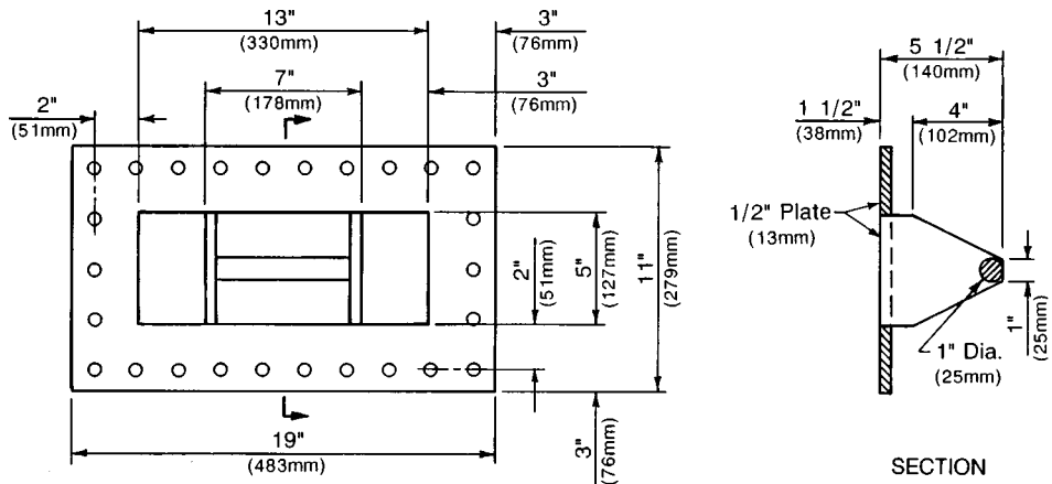
FIG. 2 Clamping Bracket
