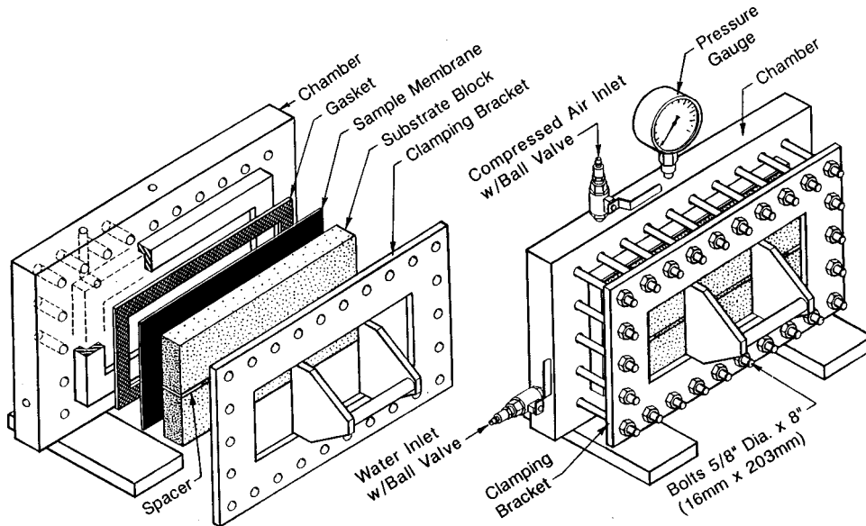
FIG. 3 Completed Assembly
