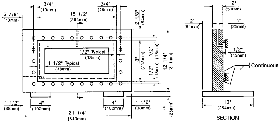
FIG. 1 Chamber
