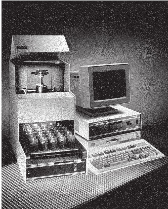
FIG. 3 Automatic Automated Cold-Cranking Simulator
