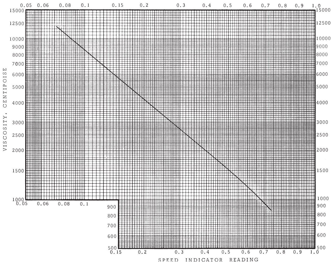
FIG. 4 Linearized Calibration Chart, Cold Cranking Simulator
