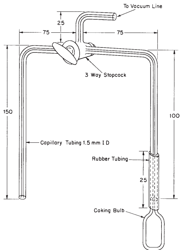
NOTE—All dimensions are in millimetres (1 in. = 25 mm). FIG. 3 Sampling Device
