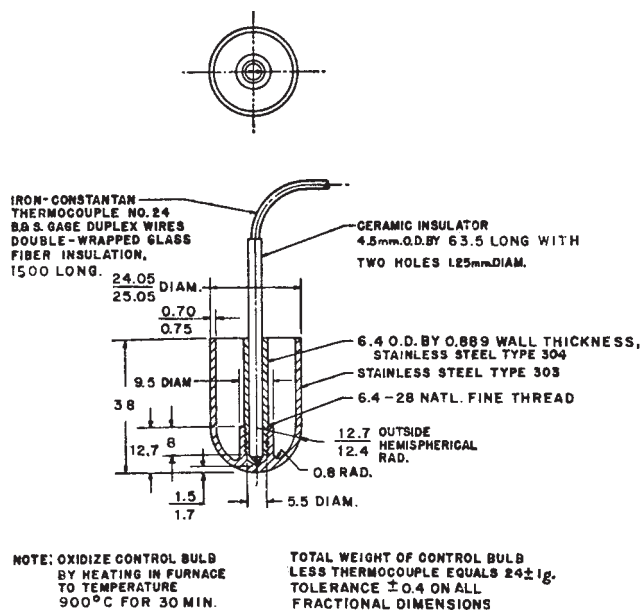
FIG. 2 Control Bulb
