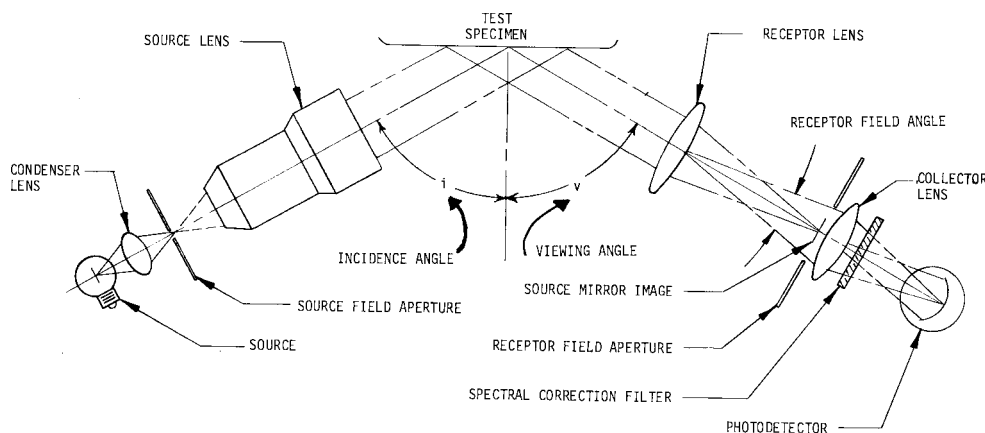
FIG. 1 Diagram of Parallel-Beam Glossmeter Showing Apertures and Source Mirror-Image Position
