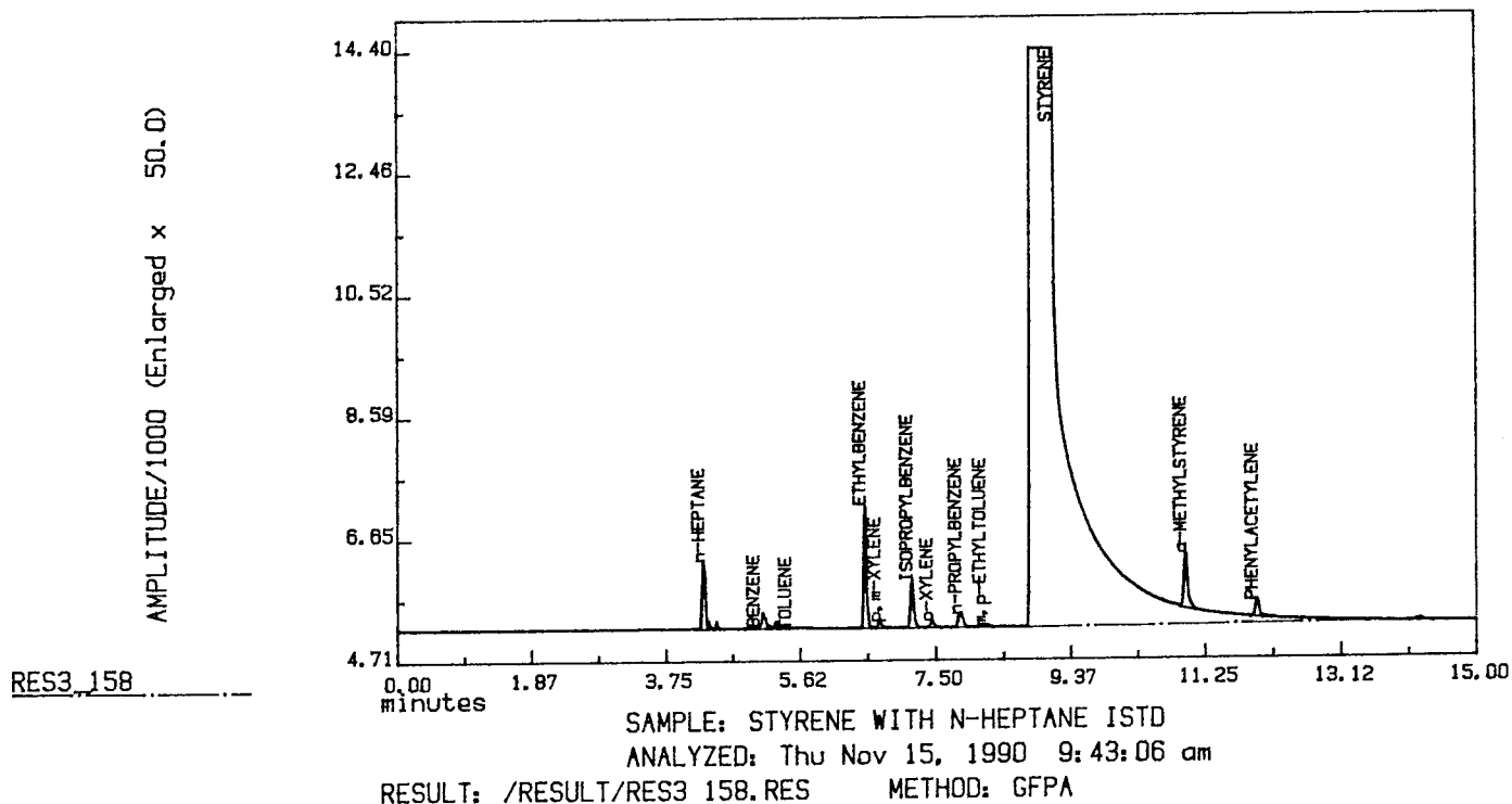
FIG. 1 Typical Chromatogram (see Table 2)
