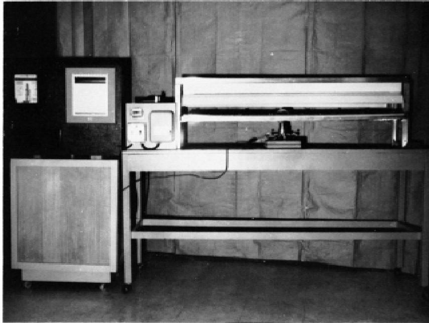
FIG. A1.3 Single-Bank Device of Four Verilux Daylight Fluorescent Lamps 6 that Handles Twenty-seven 3 by 6-in. Panels
