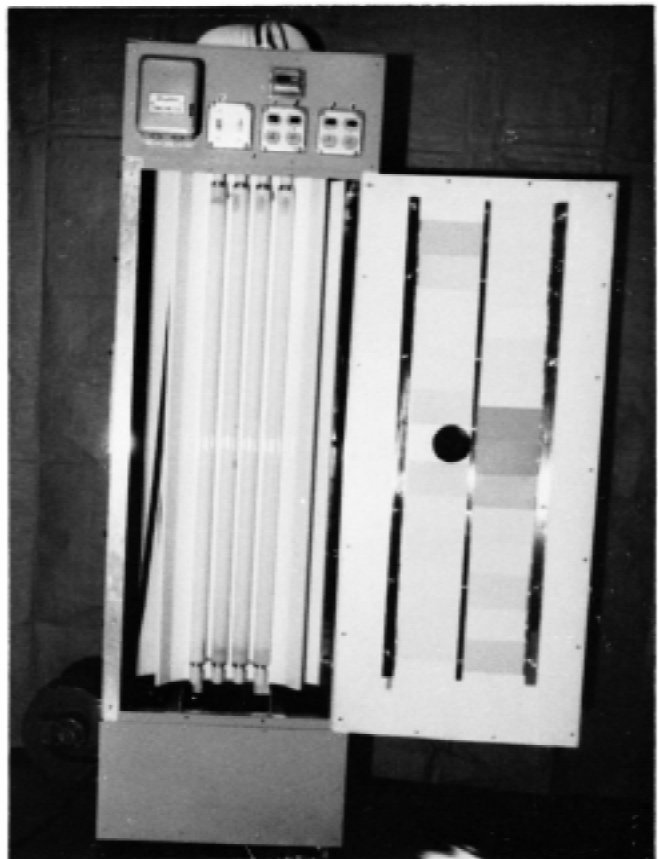
NOTE 1—Notice hole for mounting Eppley pyranometer which is attached at right. (b) Four-Bank Verilux Fluorescent Exposure Apparatus with One Panel Open
