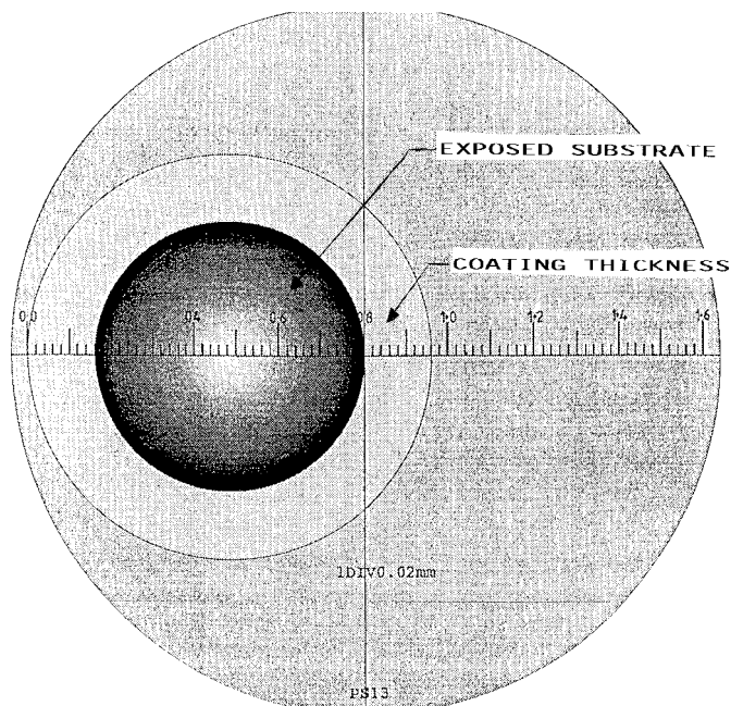
FIG. 8 Typical View Through Microscope Used with Saberg Drill
