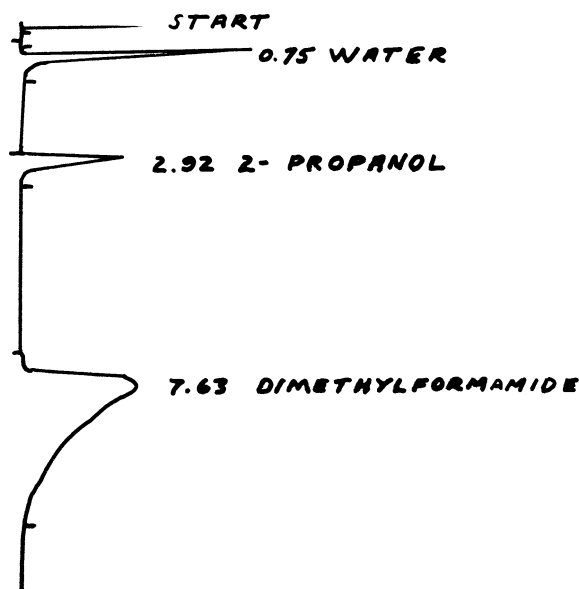
FIG. 1 Typical Chromatogram
