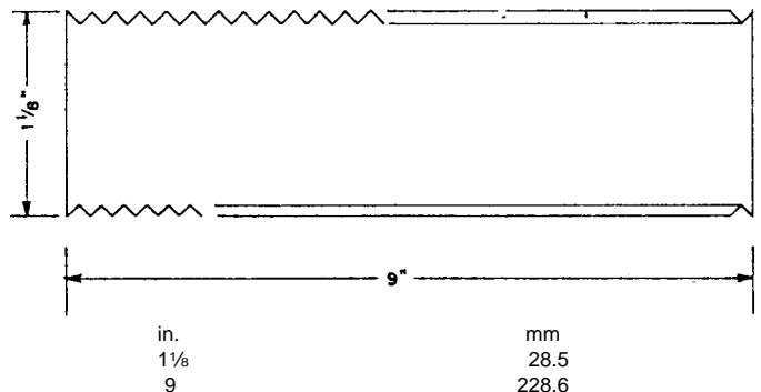
FIG. 3 Metal Test Piece Thin Film Liquid Contact
