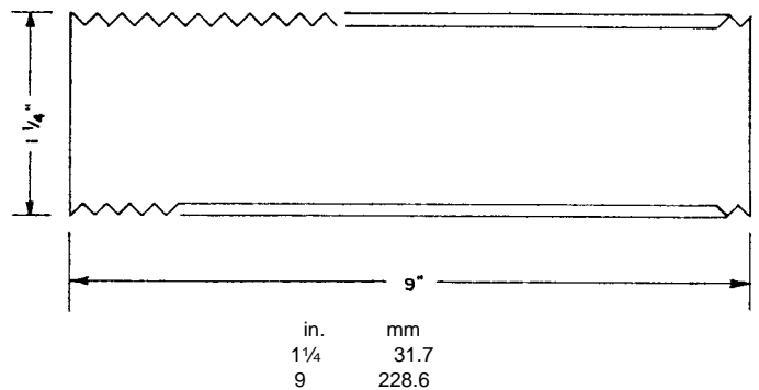
FIG. A1.2 Metal Test Piece Vapor Contact
