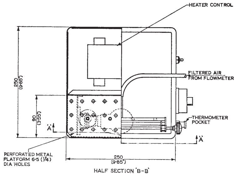
FIG. 4 Evaporation Assembly
