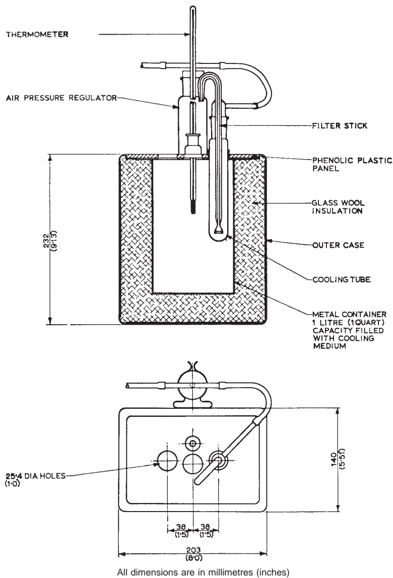
FIG. 2 Cooling Bath
