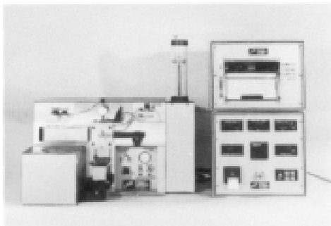
FIG. 1 Failex Block-on-Ring Test Machine with Recorder
