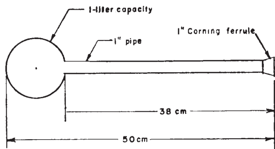
FIG. 12 Combustion Chamber
