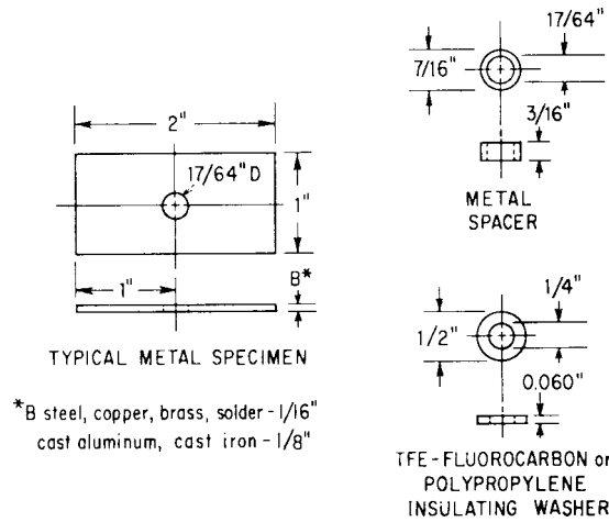
TYPICAL ASTM SPECIMEN BUNDLE A
