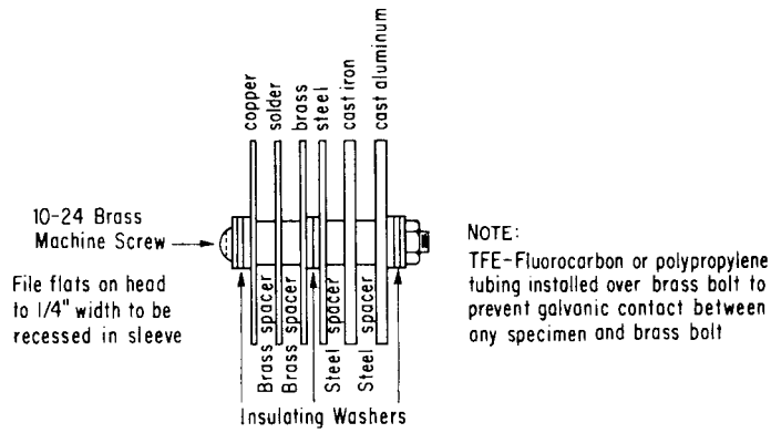
TYPICAL ASTM SPECIMEN BUNDLE A
