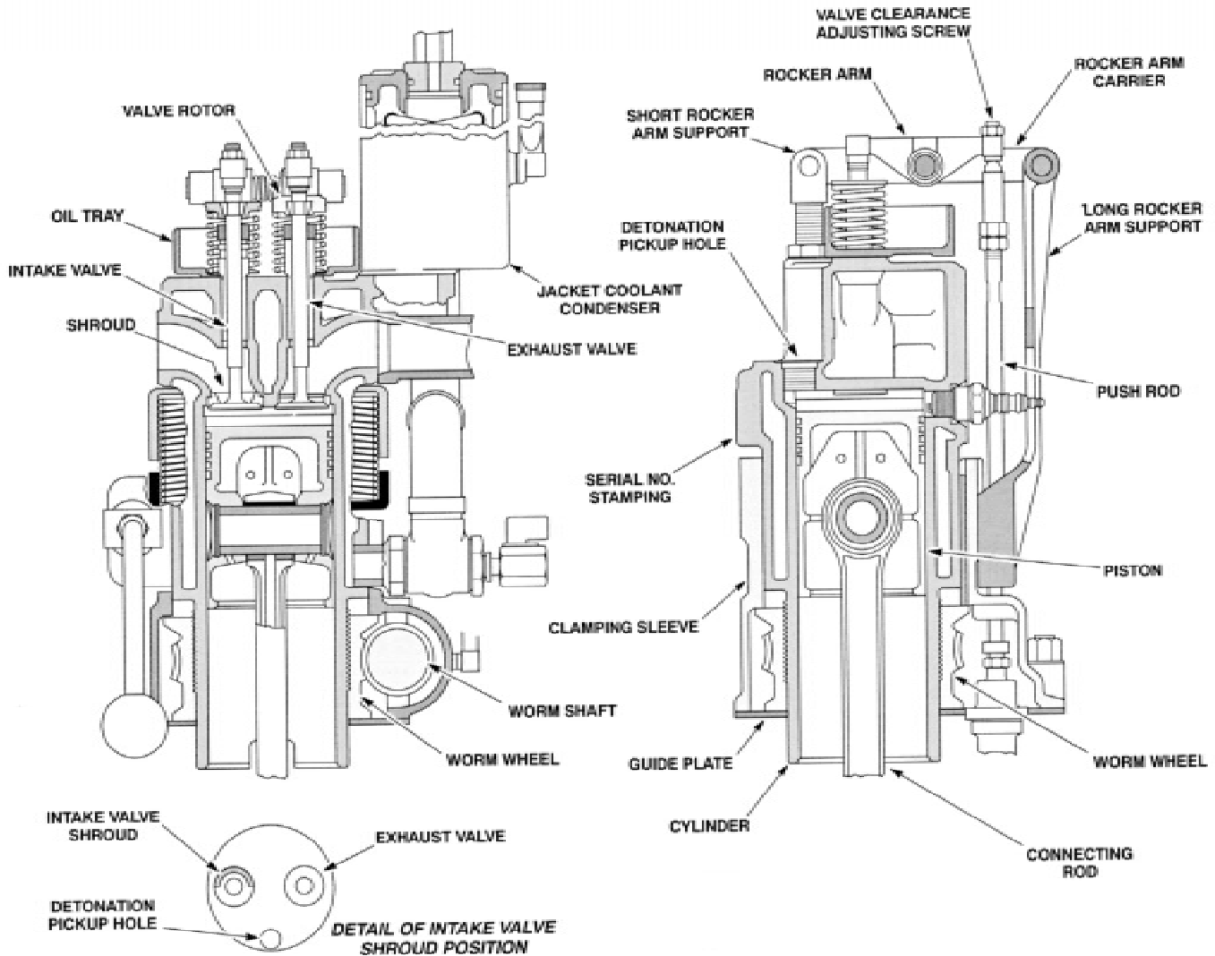
FIG. A2.2 Cylinder and Clamping Sleeve Assembly
