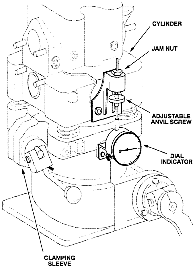
FIG. A4.3 Cylinder Height Dial Indicator
