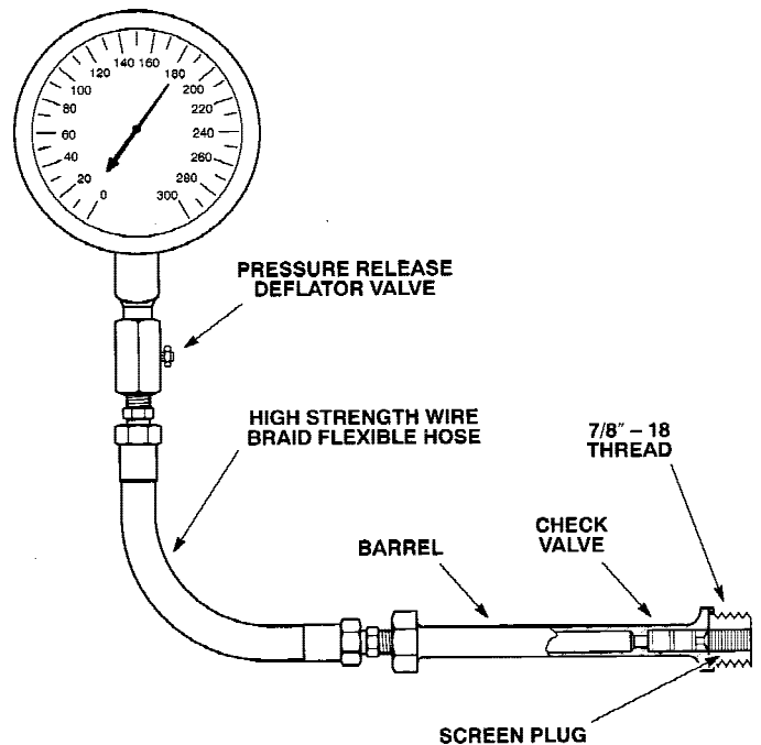
FIG. A4.4 Compression Pressure Gage Assembly
