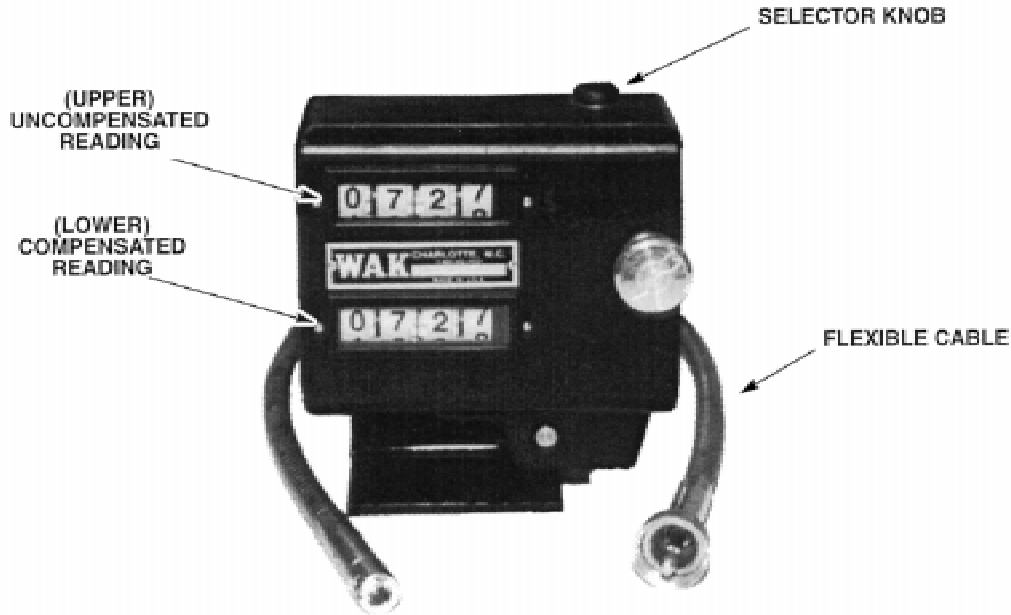
FIG. A4.2 C.R. Digital Counter
