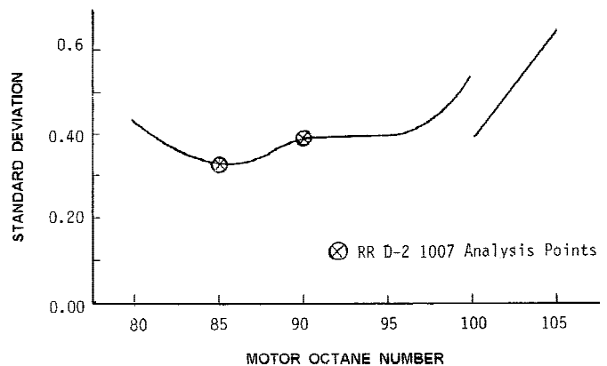
FIG. 8 Variation of Reproducibility Standard Deviation With Motor Octane Number
