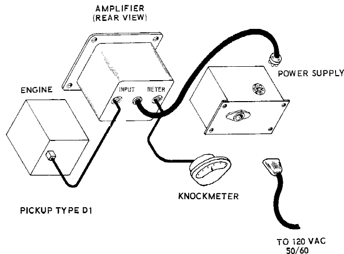
FIG. A3.1 Components of Knock Measurement Instrumentation
