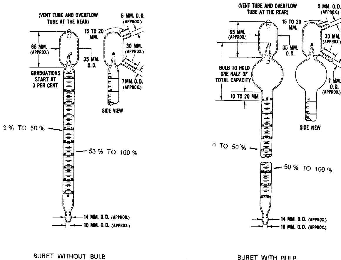
FIG. X1.2 Typical Reference Material Dispensing Apparatus Two-Buret Style
