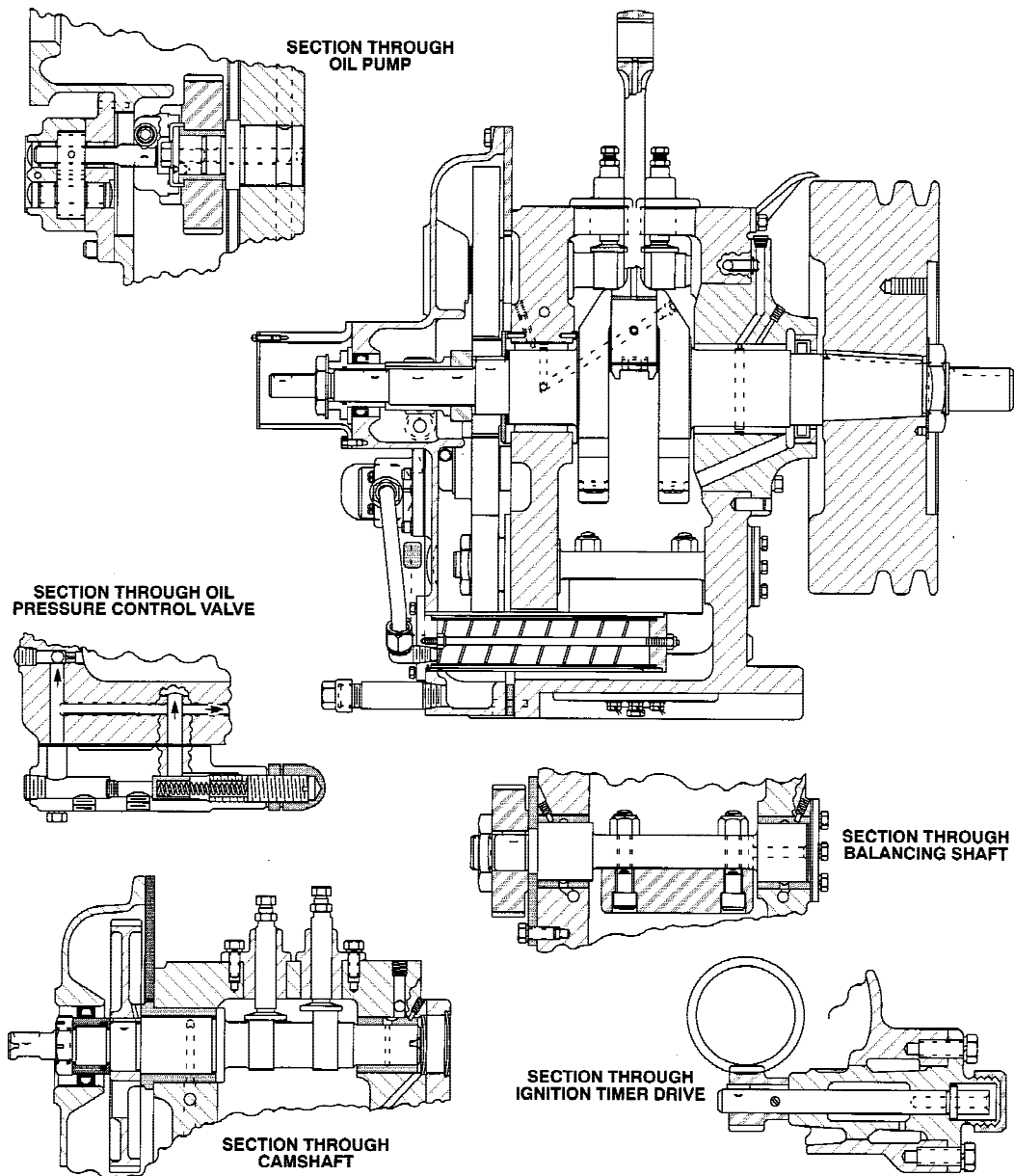
FIG. A2.1 CFR-48 Crankcase—Sectional Views
