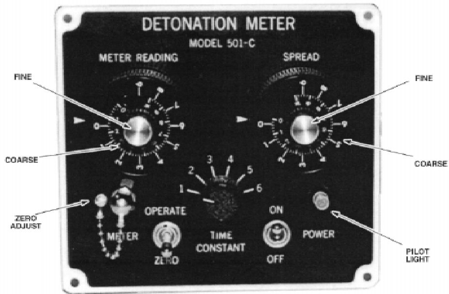
FIG. A4.7 Detonation Meter—Front Panel
