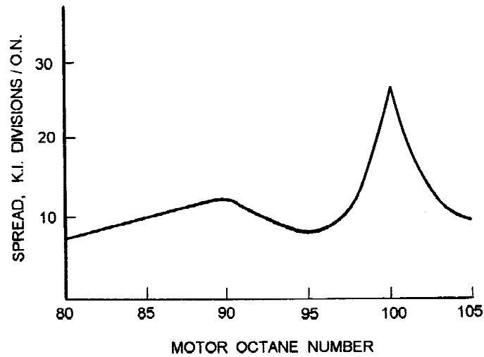
FIG. A4.6 Typical Detonation Meter Spread Characteristic
